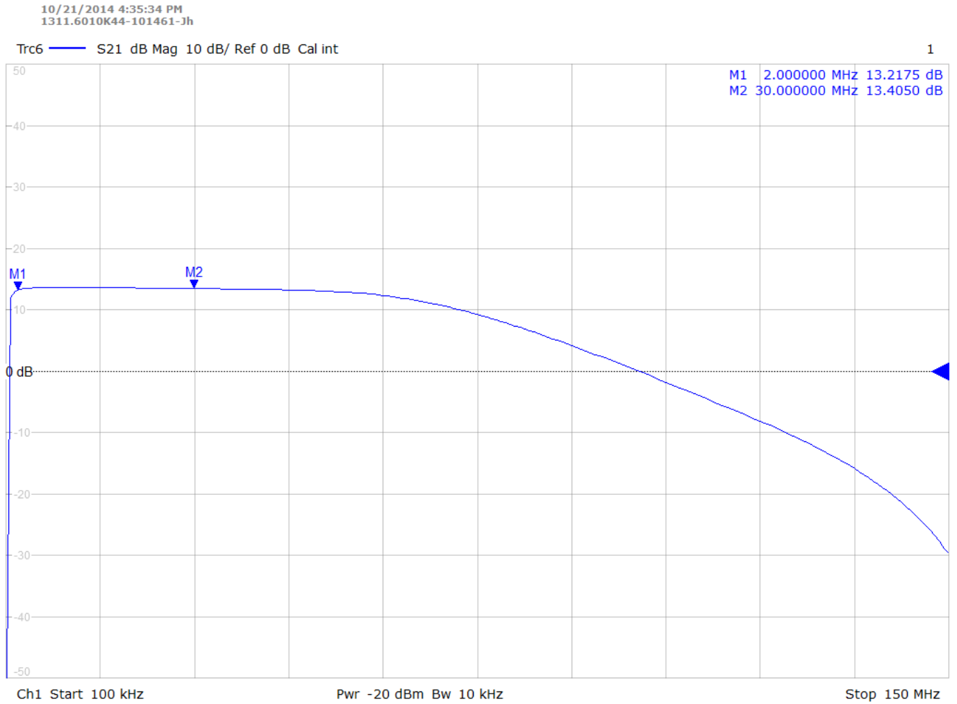
Figure 2: HF divider transfer function curve up to 150MHz
