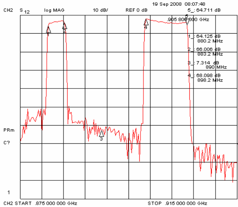
Figure 2: GR920-02 transfer function example – two independent bands on uplink frequencies.
