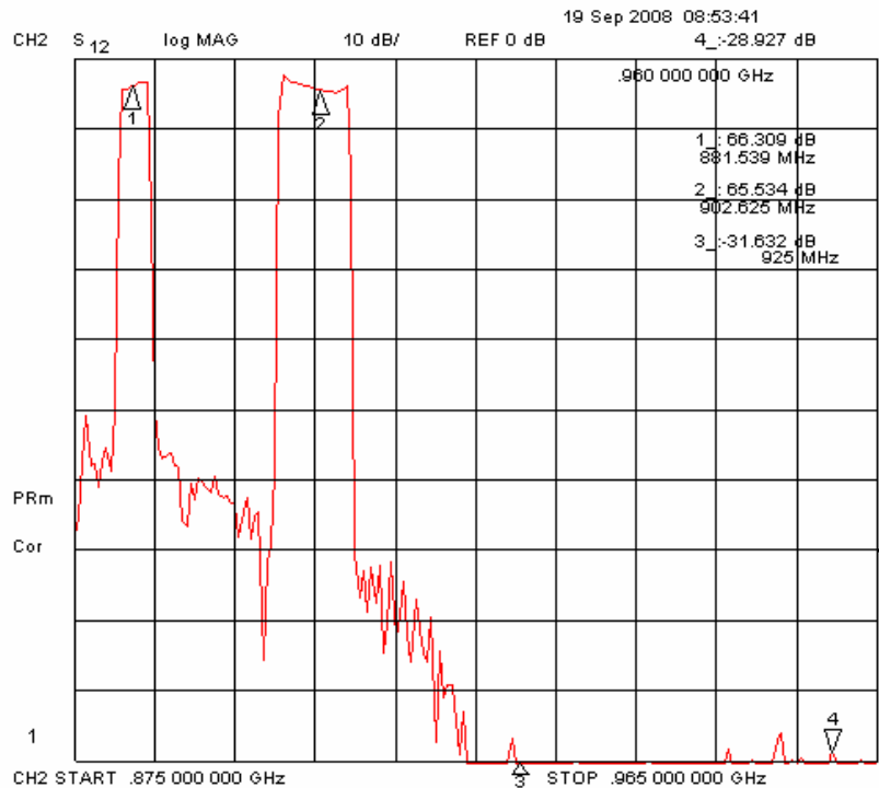
Figure 3: GR920-02 transfer function example – uplink/downlink isolation.
