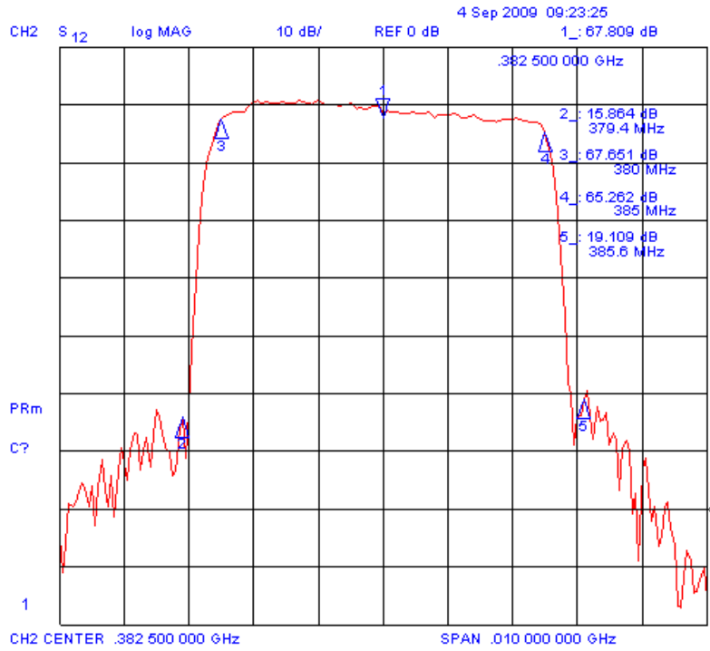
Figure 2: GR380-01 uplink transfer function example.
