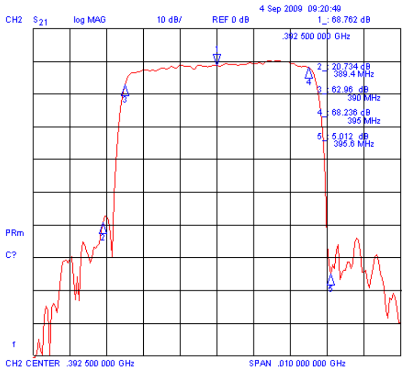
Figure 3: GR380-01 downlink transfer function example.
