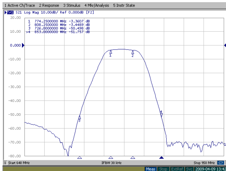
Figure 2: FB-791.25M transfer function in 640-950MHz band.
