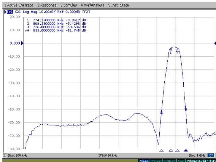
Figure 3: FB-791.25M transfer function 300kHz-1GHz band.
