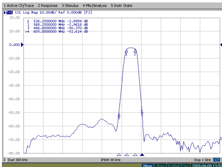
Figure 3: FB-547.25M transfer function 300kHz-1GHz band.
