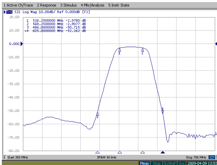
Figure 2: FB-547.25M transfer function in 350-700MHz band.
