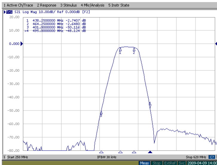
Figure 2: FB-451.25M transfer function in 250-620MHz band.
