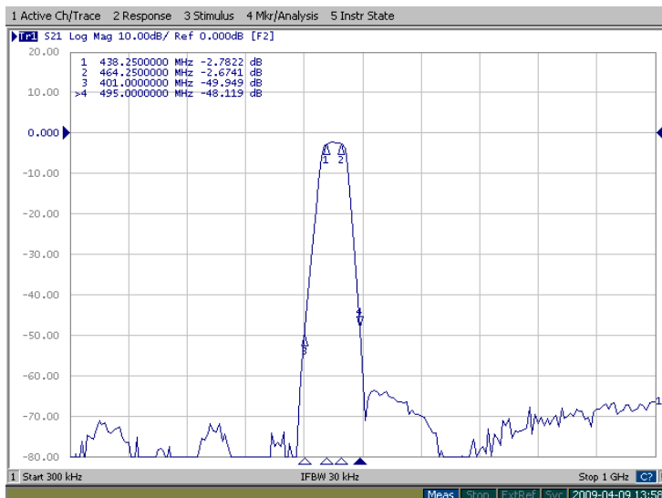
Figure 3: FB-451.25M transfer function 300kHz-1GHz band.
