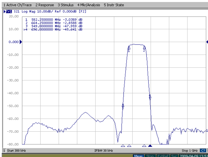
Figure 3: FB-623.25M transfer function 300kHz-1GHz band.
