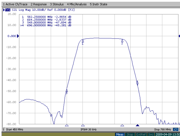
Figure 2: FB-623.25M transfer function in 450-780MHz band.
