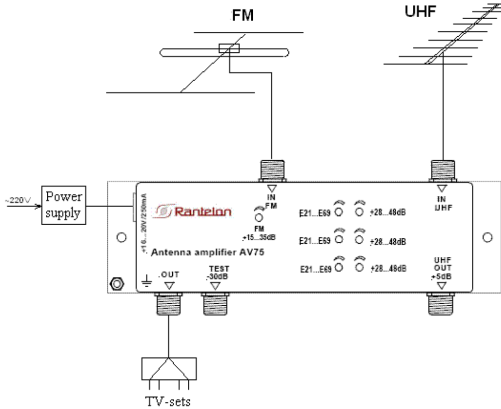
Figure 2. AV75/FM installation diagram.
