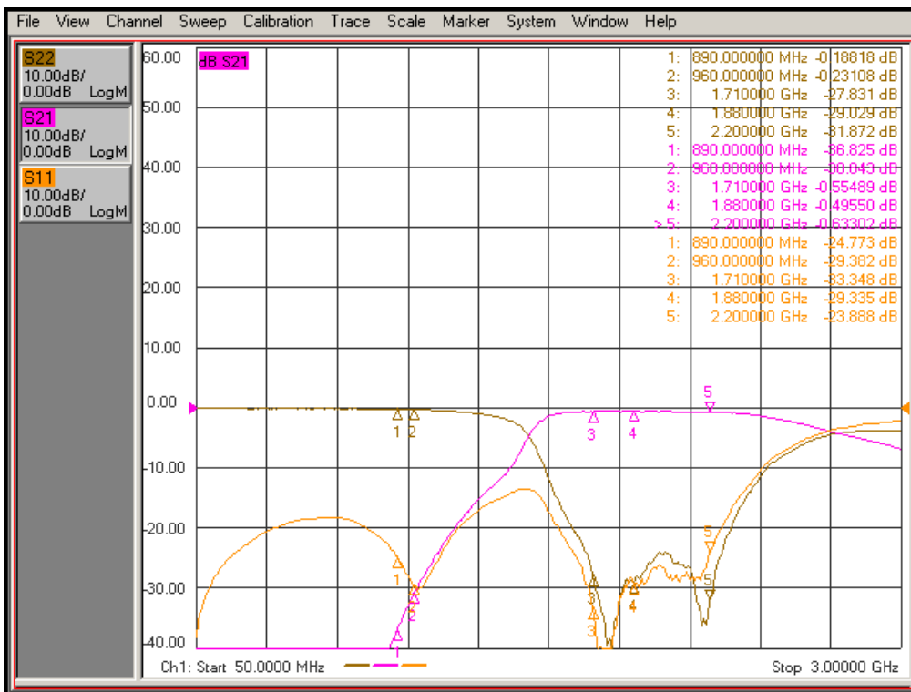
Figure 3: S11, S22 and S21 (transmission) from common port to GSM1800-UMTS port.
