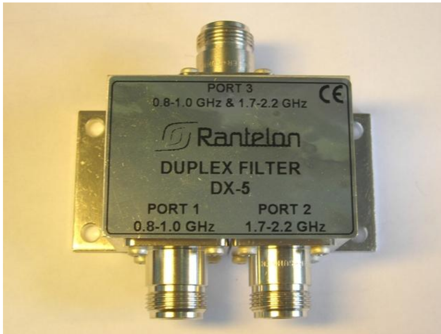
Figure 1: DX-5 Top view
