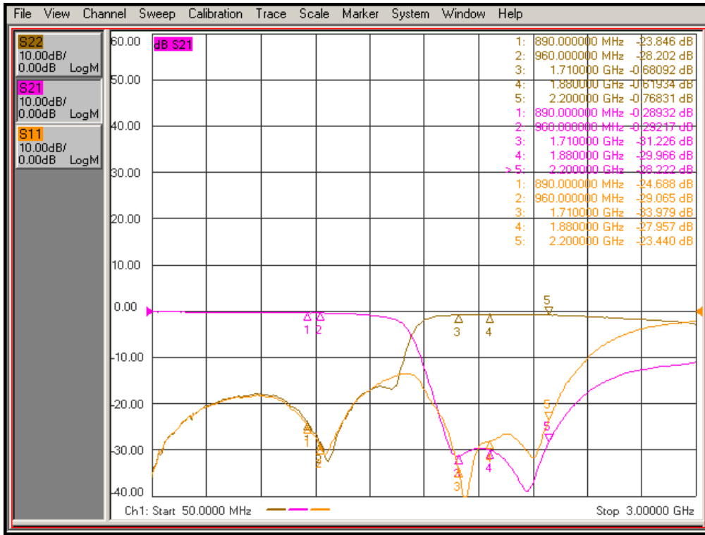
Figure 2: S11, S22 and S21 (transmission) from common port to GSM900 port.
