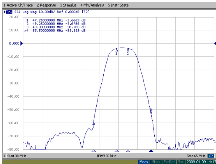
Figure 2: FB-48.25M transfer function in 30-65MHz band.
