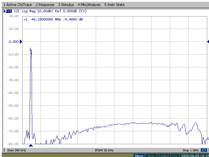
Figure 3: FB-48.25M transfer function 300kHz-1GHz band.
