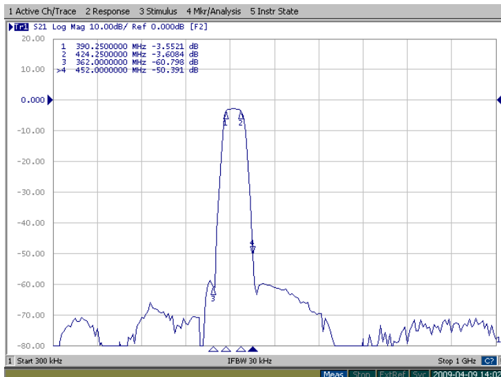
Figure 3: FB-407.25M transfer function 300kHz-1GHz band.
