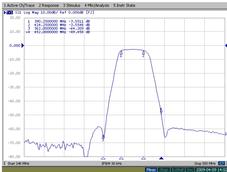
Figure 2: FB-407.25M transfer function in 240-550MHz band.
