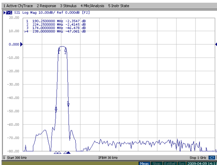
Figure 3: FB-207.25M transfer function 300kHz-1GHz band.
