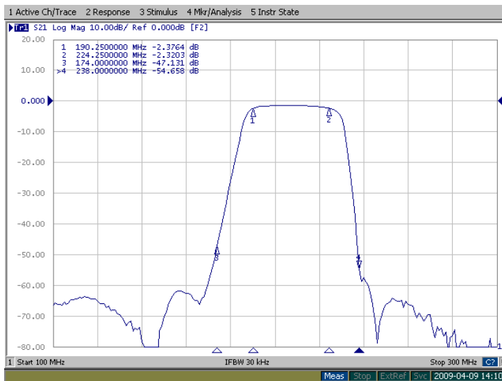
Figure 2: FB-207.25M transfer function in 100-300MHz band.
