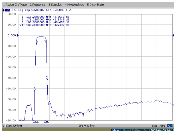
Figure 3: FB-147.25M transfer function 300kHz-1GHz band.
