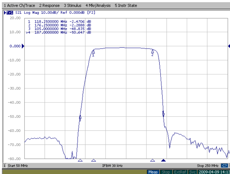
Figure 2: FB-147.25M transfer function in 50-250MHz band.
