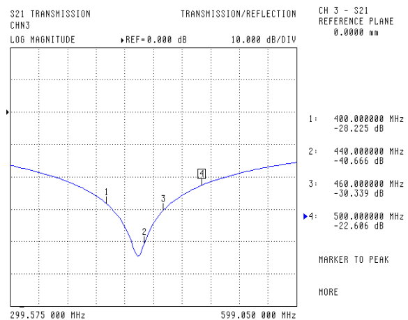
Figure 3: Example of transmission OUT<>OUT
