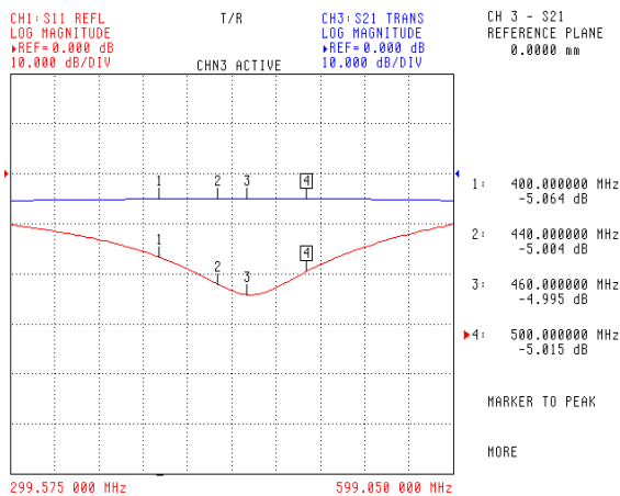
Figure 2: Example of transmission IN<>OUT and return loss (IN)
