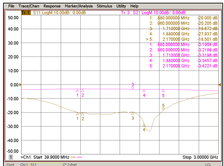
Figure 1. Example of transfer (S21) and reflection loss (-S11) functions.
