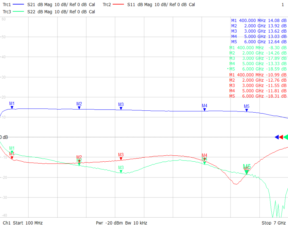
Gain(S21) and input (S11)/output(S22) matching vs. frequency
