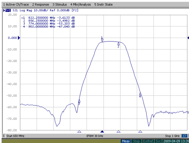
Figure 2: FB-839.25M transfer function in 650MHz-1GHz band.
