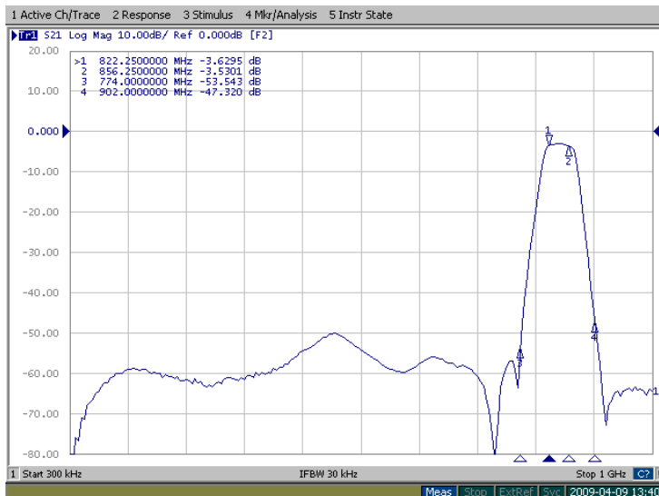
Figure 3: FB-839.25M transfer function 300kHz-1GHz band.
