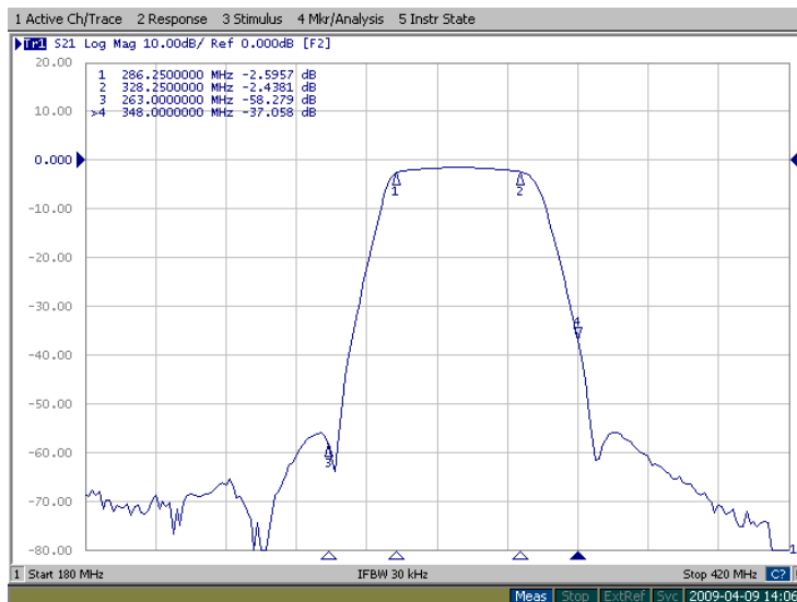
Figure 2: FB-307.25M transfer function in 180-420MHz band.
