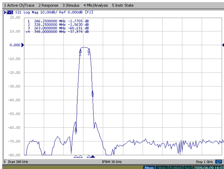
Figure 3: FB-307.25M transfer function 300kHz-1GHz band.
