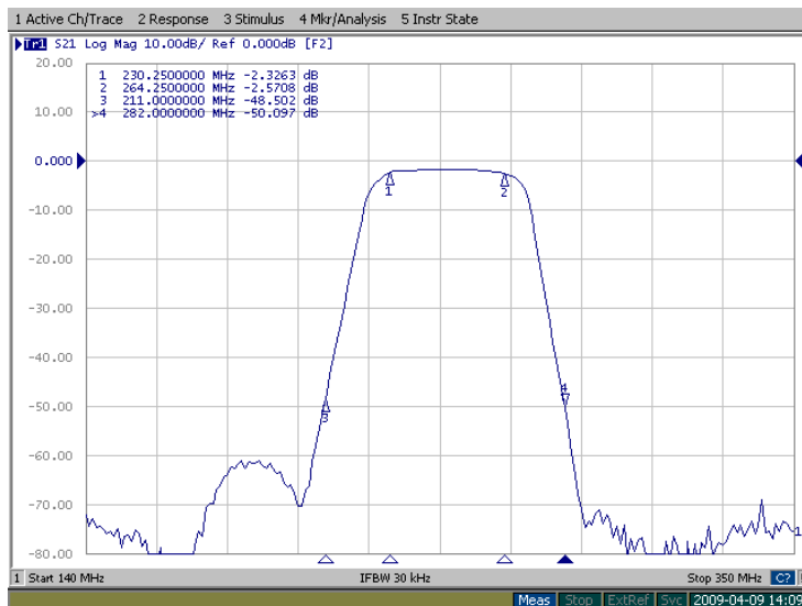
Figure 2: FB-247.25M transfer function in 140-350MHz band.
