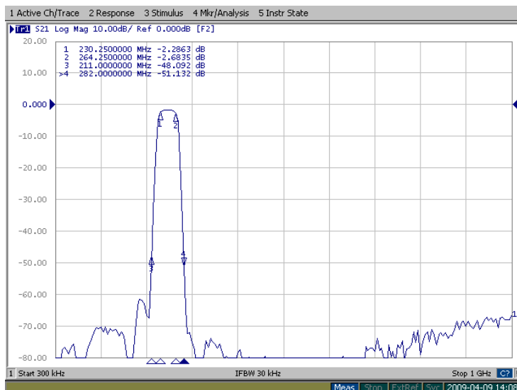
Figure 3: FB-247.25M transfer function 300kHz-1GHz band.
